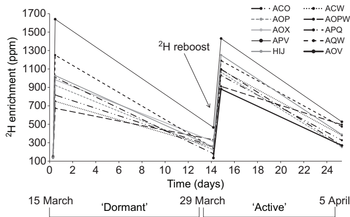
Fig. 2. Deuterium enrichment values of 10 dormant (15–29 March) and active (29 March to 5 April) female terrapins. Enrichment levels given at day 0 (15 March 2012) are background ^2\text{H} deuterium ( E_{\text{wat}} ) and equilibration ( E_{\text{mix}} ). Enrichment levels given at day 14 (29 March 2012) are E_{\text{final}} and E_{\text{mix}} after ^2\text{H} deuterium reboost. Enrichment levels at day 25 (5 April 2012) are E_{\text{final}} . All terrapins were buried immediately prior to initial injection of ^2\text{H} deuterium on 15 March 2012 (i.e. 'dormant'), but terrapins began to emerge from dormancy during late March/early April 2012 (between 29 March and 5 April, i.e. 'active'). Turtle ID (3-letter code) is given in the key.
