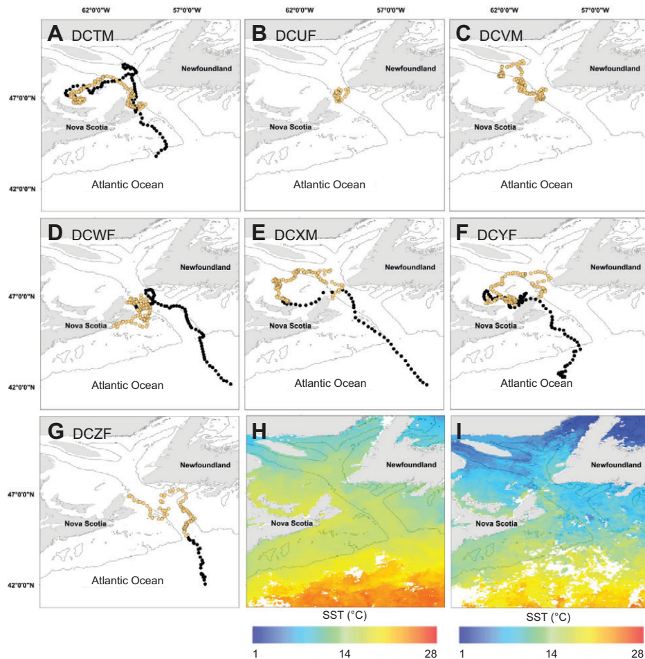
Fig. 1. State space model (SSM) tracks of leatherback sea turtles tracked offshore Eastern Canada. (A–G) Tracks show resident (yellow circles) and post-resident (black circles) periods of leatherback turtles in Canadian waters north of 42°N. Monthly mean sea surface temperature (SST) data for September (H) and October (I) of 2009 were recorded by Advanced Very High Resolution Radiometer (AVHRR) onboard NOAA Polar-orbiting Operational Environmental Spacecraft (Pathfinder Version 5, 4.4 km resolution). DC identifiers correspond to different turtles.
