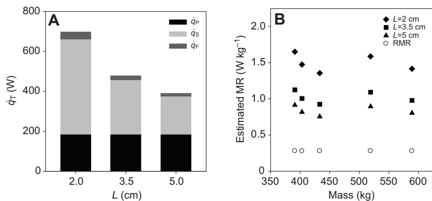
Fig. 4. Estimates for total heat transfer and metabolic rate of leatherback sea turtles at high latitude. (A) Estimates of total heat transfer ( \dot{q}_T ) represented as the sum of heat transferred to ingested prey ( \dot{q}_p ) and heat loss across the shell ( \dot{q}_s ) and flippers ( \dot{q}_f ) at various values for insulation (fat) thickness L . In order to maintain a thermal gradient, rates of metabolic heat production must equal \dot{q}_T . (B) Estimated mass-specific metabolic rate (MR) based on \dot{q}_T for five leatherbacks during the resident period assuming an insulation thickness L of 2, 3.5 and 5 cm. Resting metabolic rate (RMR) was calculated as \text{RMR} = 0.768 \text{ mass}^{-0.169} (Wallace and Jones, 2008).
